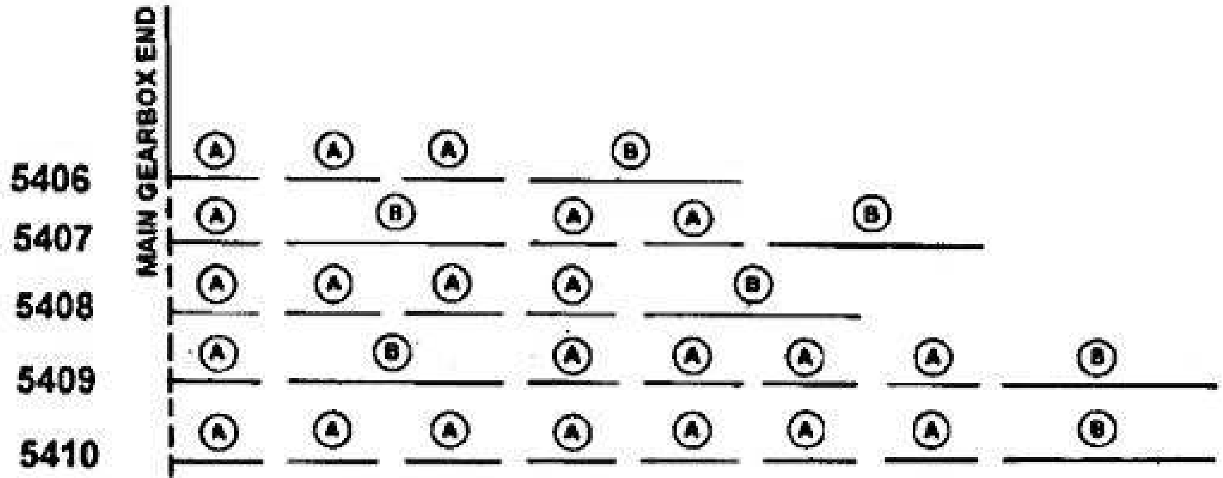
SEGMENTED SHAFT LOCATIONS
